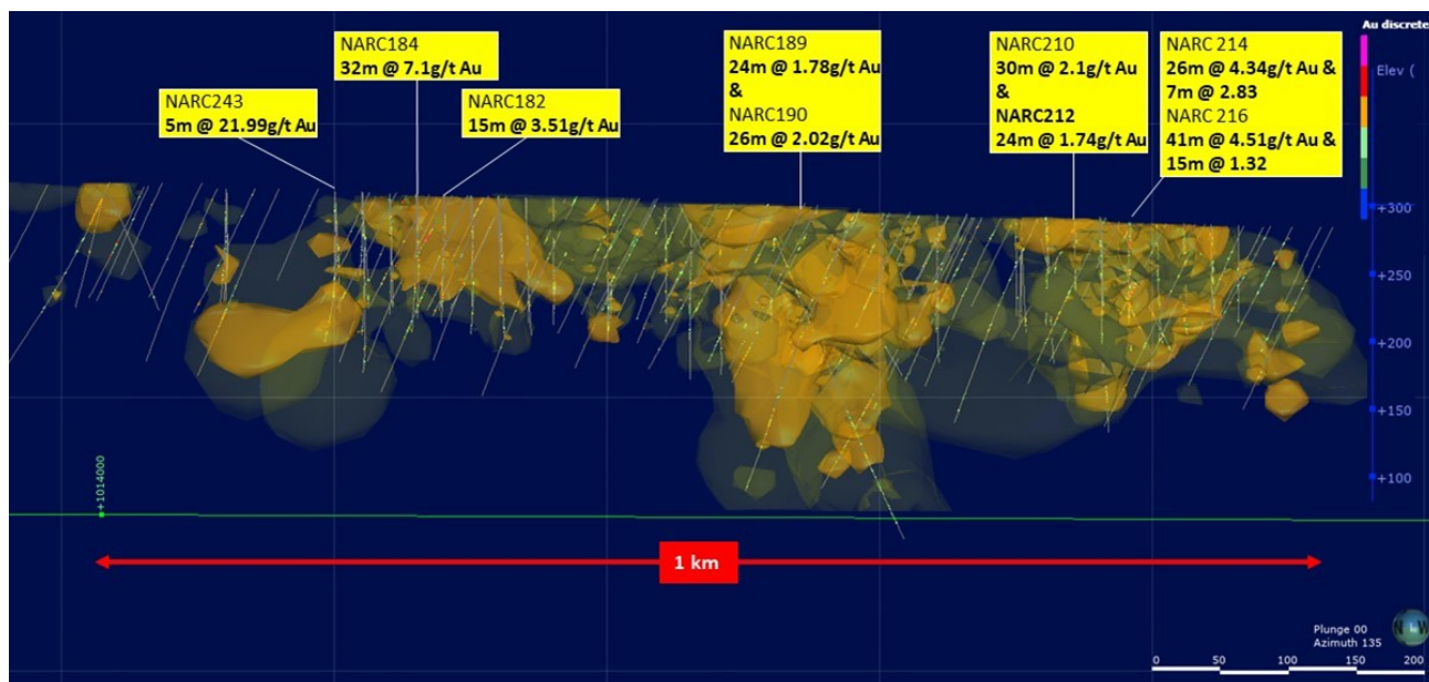
Figure 3: Long section of updated 3D exploration model looking SE on the Tchaga Prospect 2 with select drill intercepts from the reporting period - note the four lobes (refer to Figure 2) and the northern-most lode which has had limited drilling – (gold colour is 0.5g/t Au cut-off and green is 0.2g/t Au cut-off)
