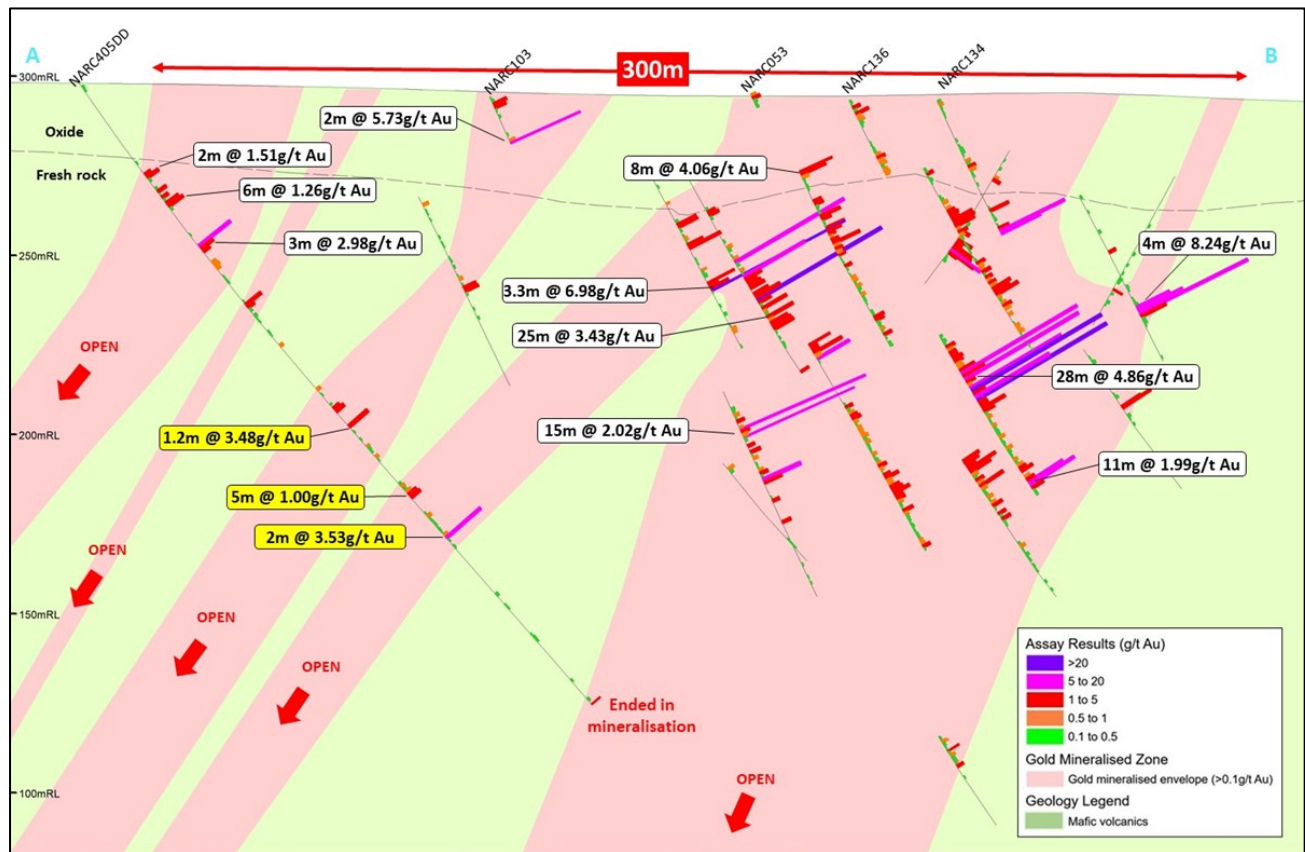
Figure 2: Section AB looking northeast showing new (yellow) and previous 2 (white) drill results – note that the new drilling results from NARC405DD extend mineralisation to the SW from previously reported high-grade zones.
